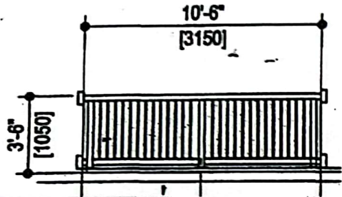
ELEVATION OF RAILING (BALCONY)
